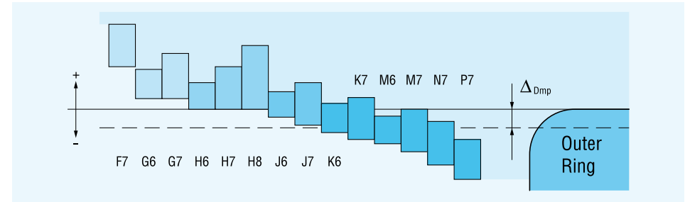
Bore Diameter Tolerance Limiting Deviations
